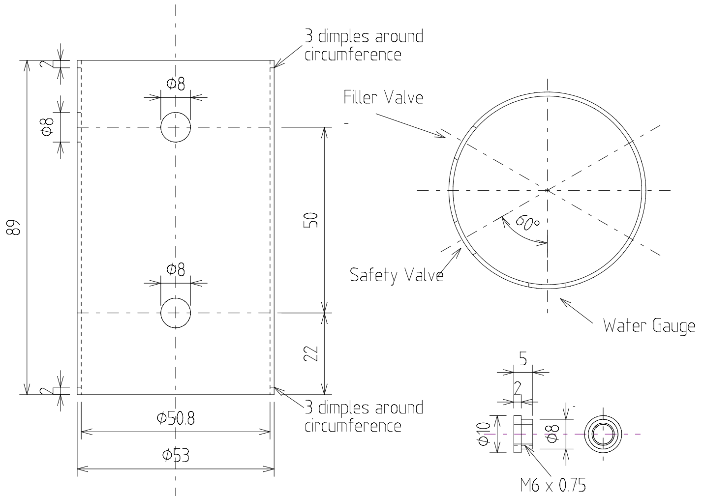
Boiler Shell (#88)
