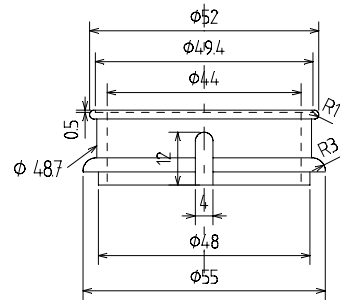
Smokebox Ring (#101)
